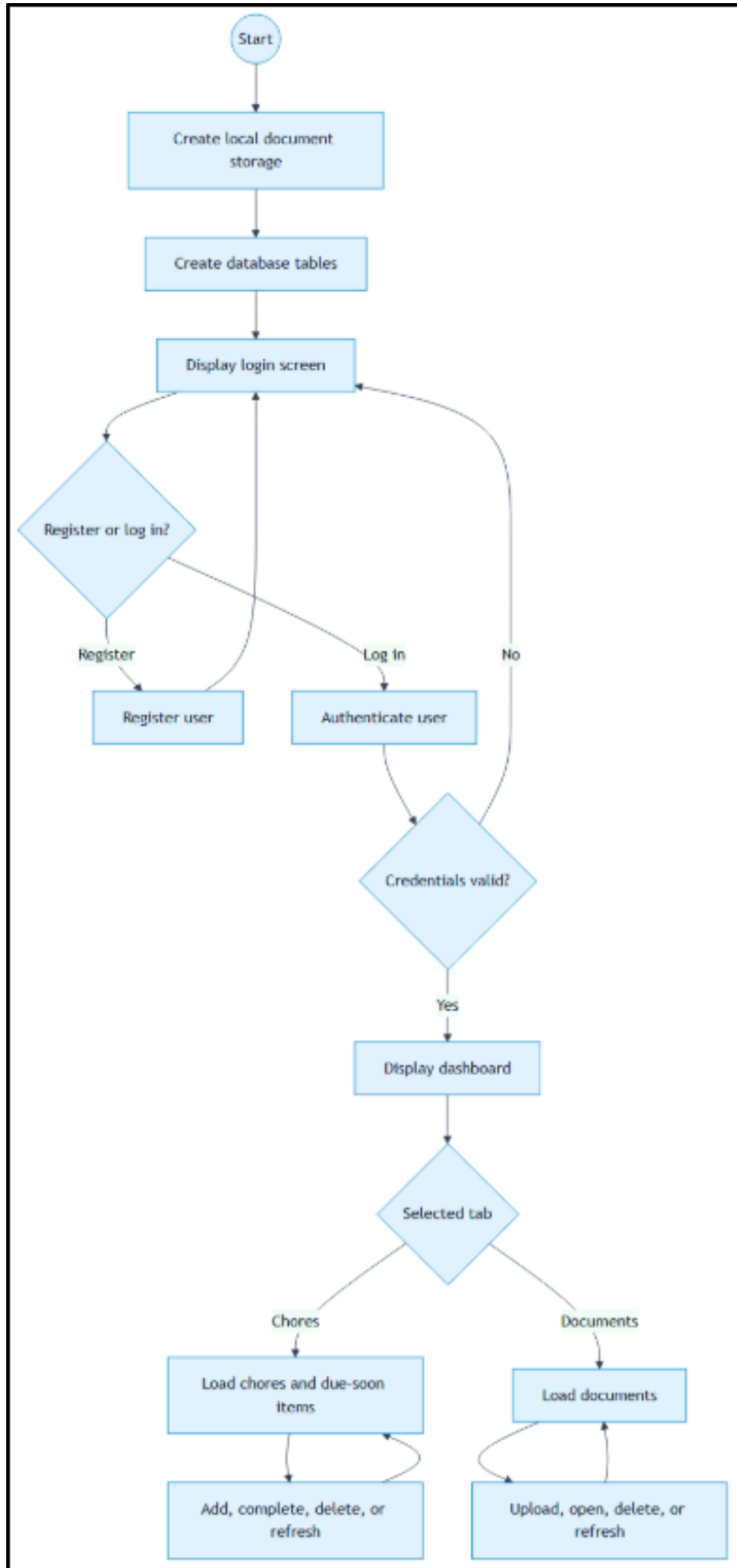
Figure: LifeAdmin Activity Diagram
